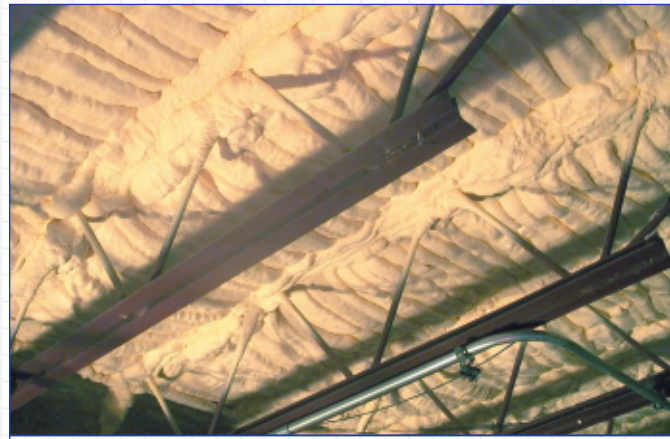
Area of application for Icynene® included the footprint of the chillers and walk-in freezers plus a perimeter area extending 10 feet beyond.
