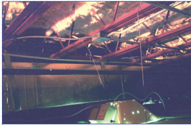
Icynene® insulation applied directly to the metal ceiling area below the chillers and walk-in freezers.
